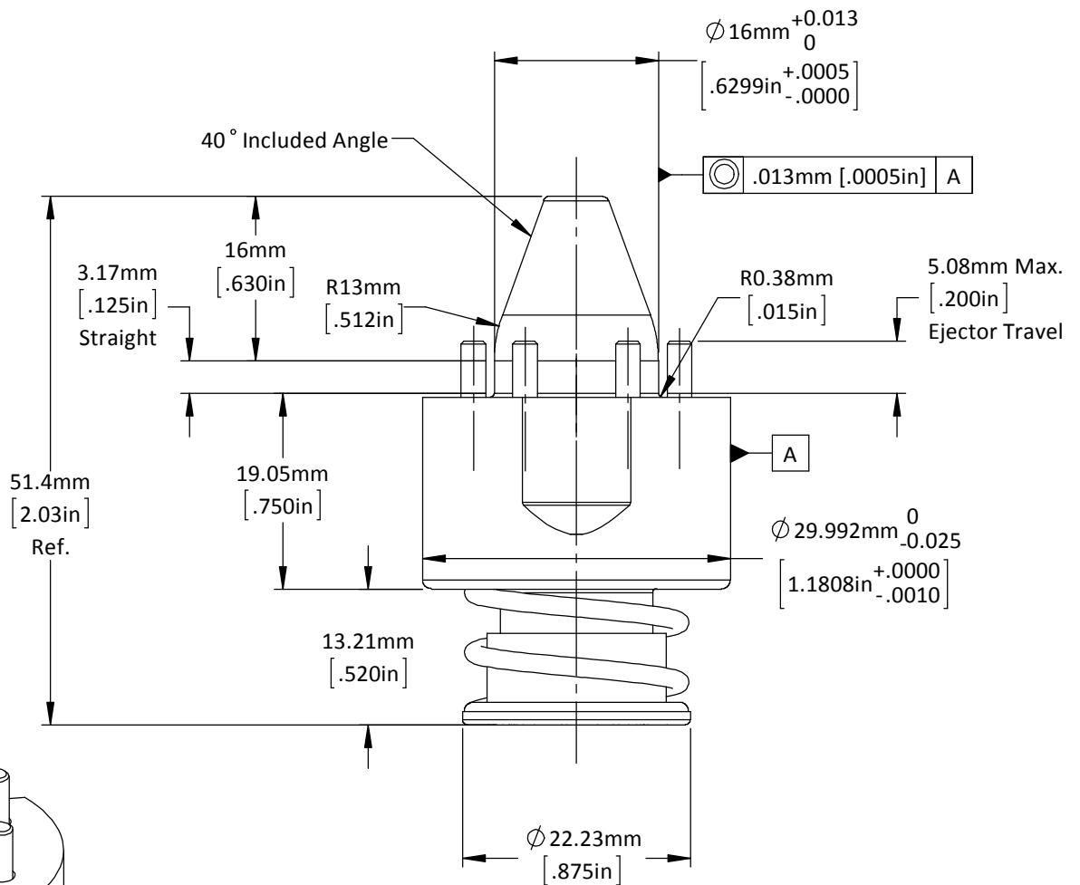
1 Hold Down PA-16mm-3.2mm-L-P-F1
