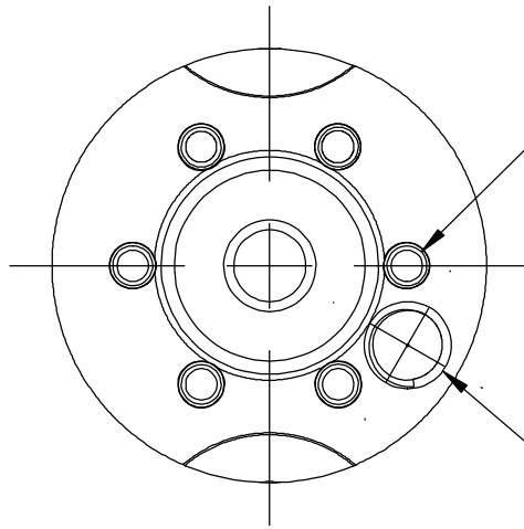
2 Hold Downs PA-13mm-2.5mm-L-P-F2
