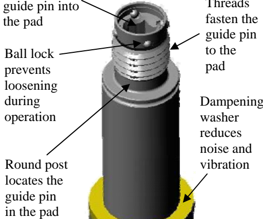
GK100 Guide Pin
